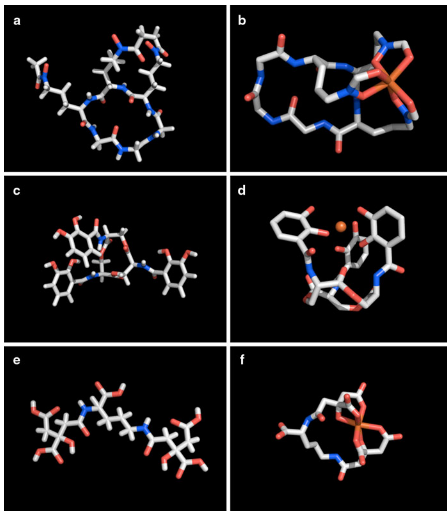
Fig. 1 Crystal structures of three representative siderophores: enterobactin, ferrichrome and staphyloferrin A are depicted without ( left side ) and with Fe 3+ bound ( right side ). Ferrichrome ( a and b ), a hydroxamate type siderophore, is produced by the fungus Ustilago sphaerogena . Enterobactin
